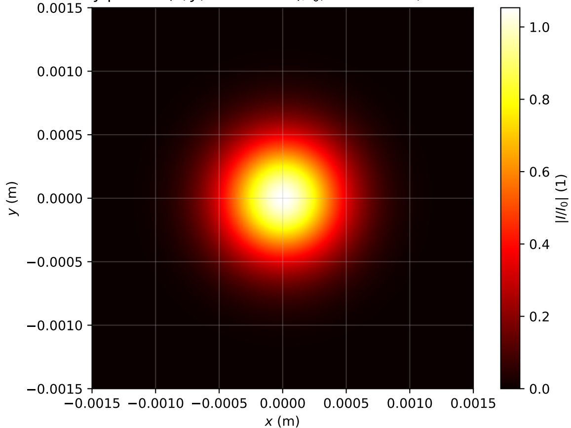
Intensity profile I(x, y, z = 0.318m)/I_0 , P_{in}=0.8P_{cr} , artificial time
